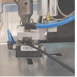
Ultrasonic welding
