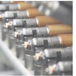
Winding of coils
